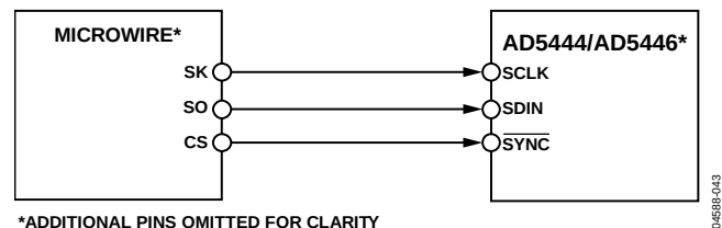
Figure 52. MICROWIRE to AD5444/AD5446 Interface
