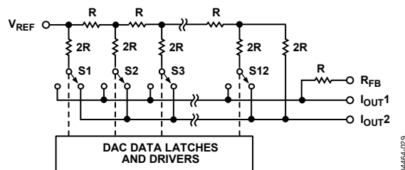
Figure 37. Simplified Ladder
