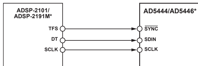
Figure 47. ADSP-2101/ADSP-2191M to AD5444/AD5446 Interface
