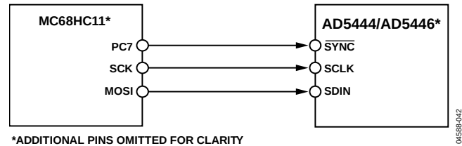
Figure 51. MC68HC11 to AD5444/AD5446 Interface
