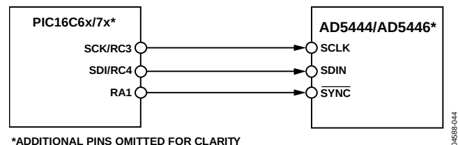
Figure 53. PIC16C6x/7x to AD5444/AD5446 Interface
