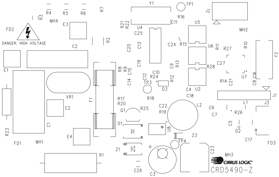
Figure 45. Silkscreen
