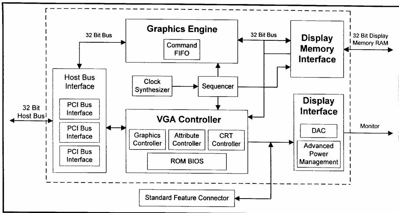
TGUI9440-R Block Diagram
