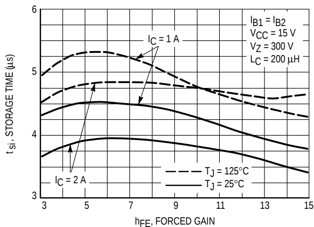
Figure 11. Inductive Storage Time, t_{sj} ( h_{FE} )
