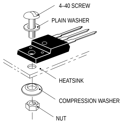
Figure 27a. Screw-Mounted
