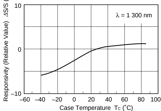
TEMPERATURE DEPENDENCE OF RESPONSIVITY
