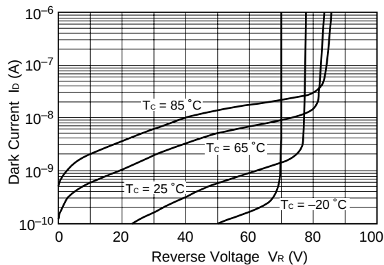
DARK CURRENT vs. REVERSE VOLTAGE
