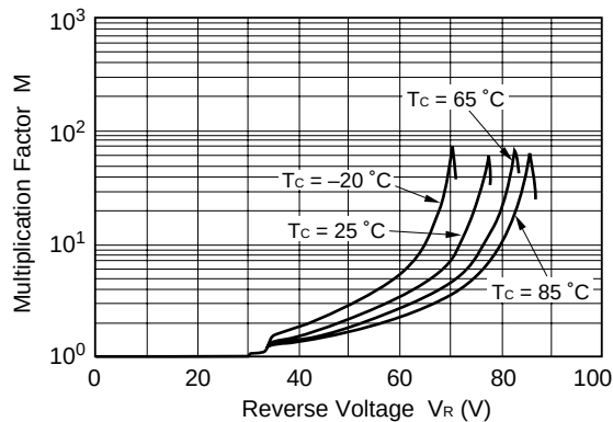
MULTIPLICATION FACTOR vs. REVERSE VOLTAGE
