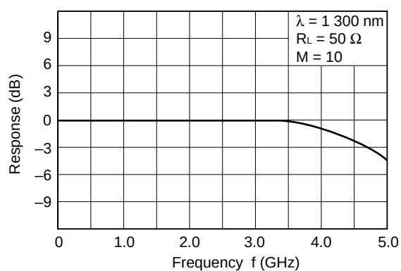
FREQUENCY RESPONSE
