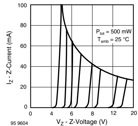
Fig. 6 - Z-Current vs. Z-Voltage
