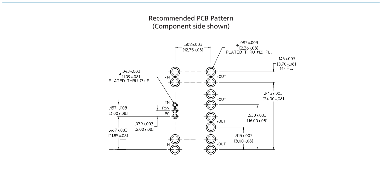
Figure 19 — PCB mounting specifications
