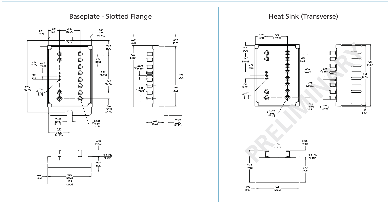
Figure 18 — Module outline
