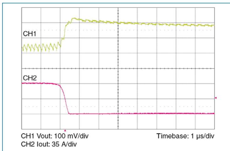
Figure 11 — 70-0 A load step with 100 \mu F input capacitor and no output capacitor.
