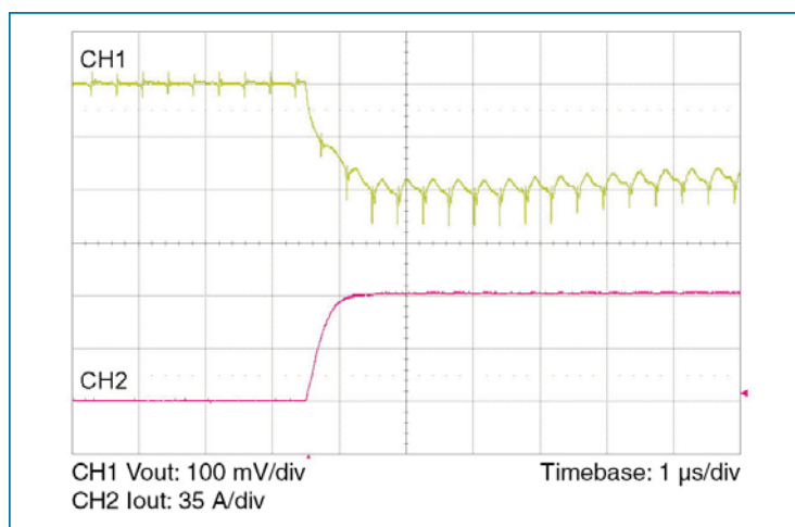
Figure 10 — 0-70 A load step with 100 \mu F input capacitor and no output capacitor.
