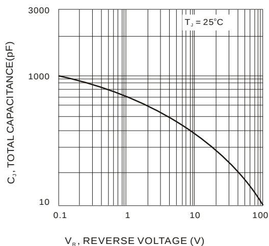
Fig.5-TYPICAL TOTAL CAPACITANCE
