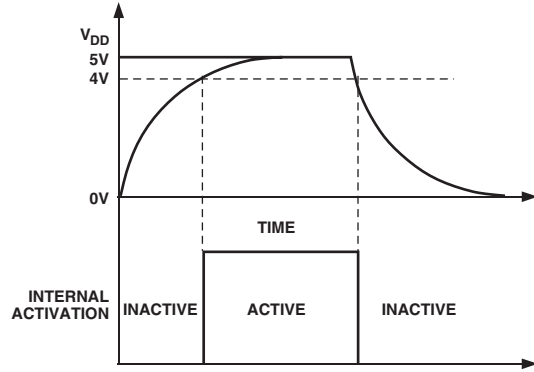
Figure 9. On-Chip Power Supply Monitor
