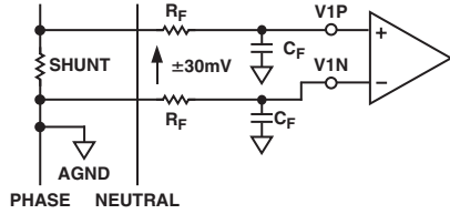
Figure 7. Typical Connection for Channel V1
