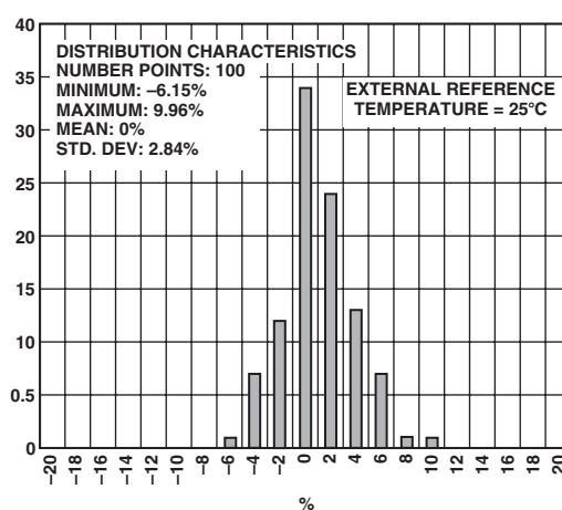
TPC 10. Part-to-Part CF Distribution from Mean
