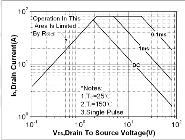
Fig. 10. Maximum safe operating area(TO-263)
