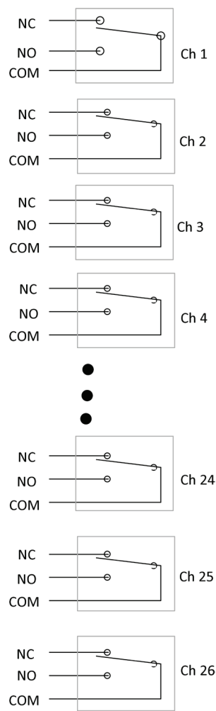
Figure 2. M9130A 26-ch, SPDT, armature relays
