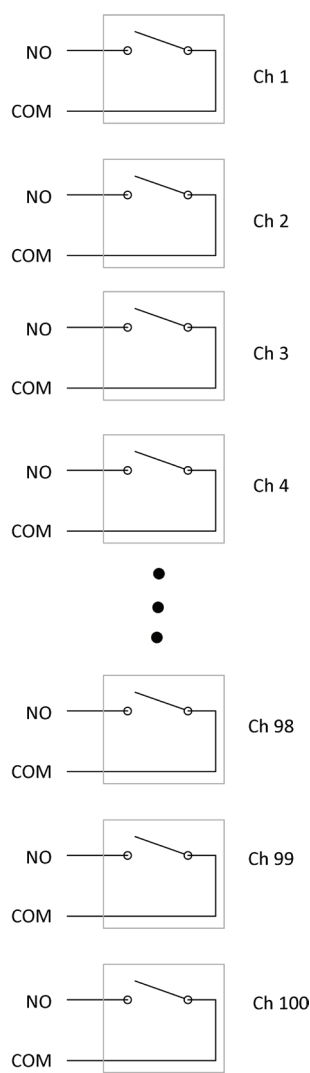
Figure 8. M9135A 20-ch, SPST, 10A, 300W
