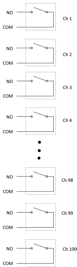
Figure 7. M9133A 100-ch, SPST, reed relays
