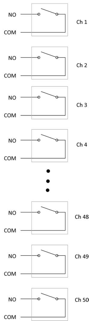
Figure 6. M9132A 50-ch, SPST, reed relays.
