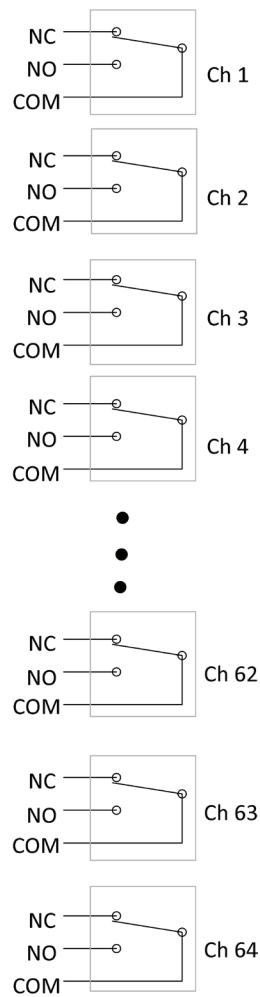
Figure 4. M9131A 64-ch, SPDT, reed relays
