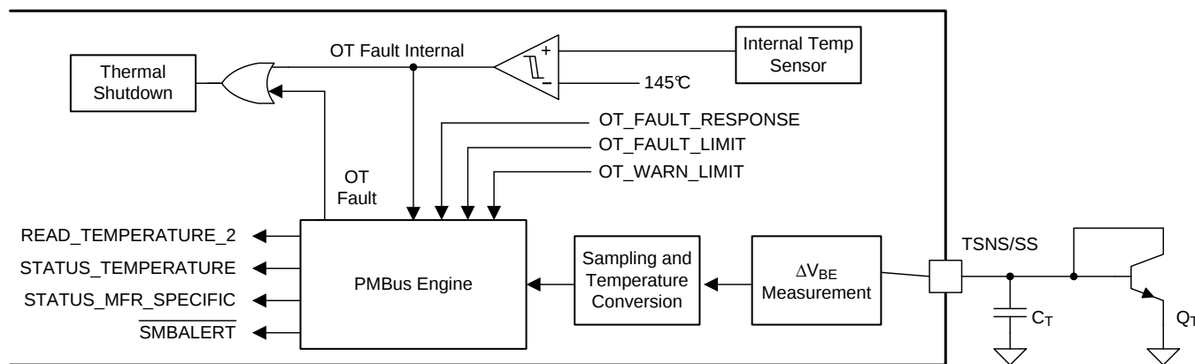
Figure 38. Over-Temperature Protection
