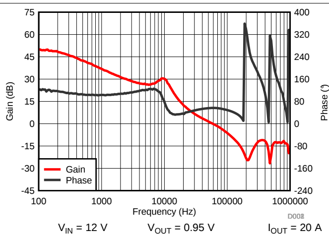
Figure 48. System Bode Plot
