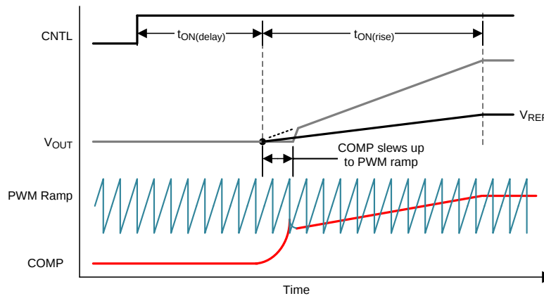
Figure 36. Soft-Start Timing
