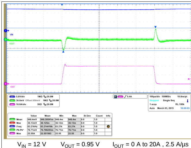
Figure 51. Transient Load
