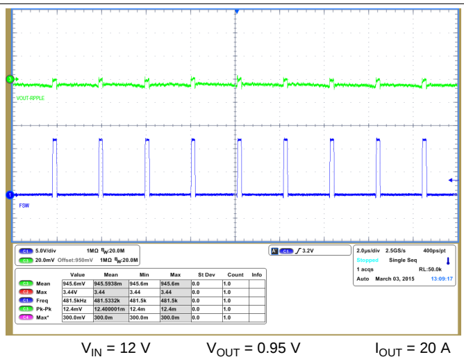
Figure 52. DC Ripple
