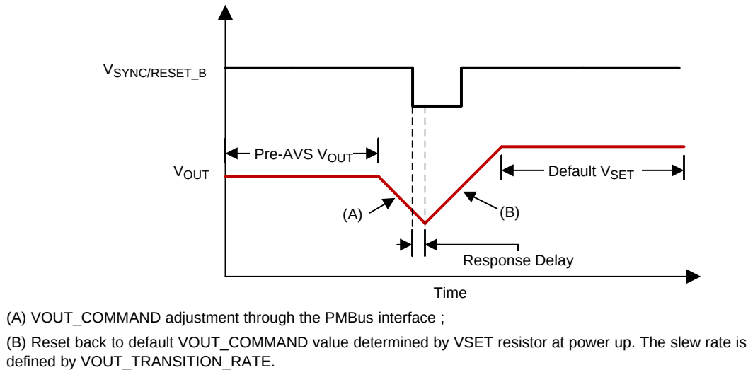
Figure 35. Output Voltage Reset
