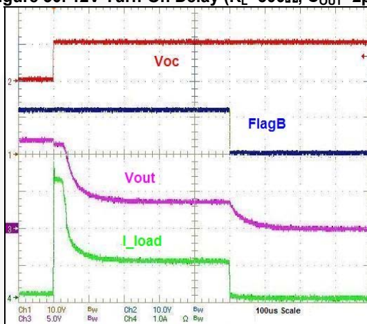
Figure 32. 12V Blanking Time (Output Overloaded and t_{blank} Expired, FPF2700/01, I_{LIM}=1A , I_{LOAD}=3.3A , C_{OUT}=2\mu F , R_{LOAD}=500\Omega ) V_{OC}^{(2)}
