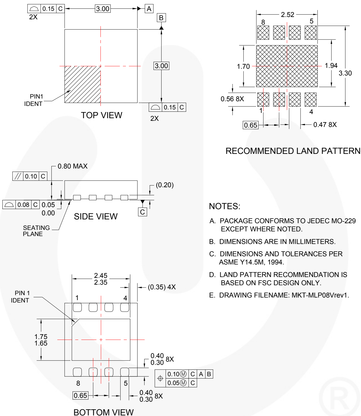
Figure 1. 8-Lead, 3x3mm Molded Leadless Package (MLP)
