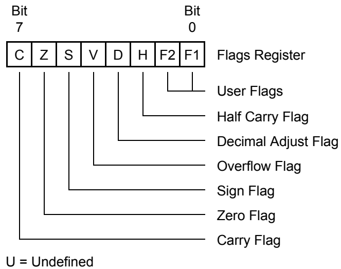
Figure 56. Flags Register
