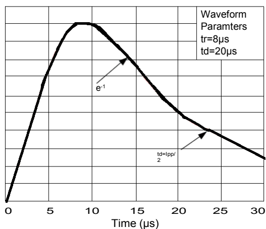
Figure3:Pulse aveform
