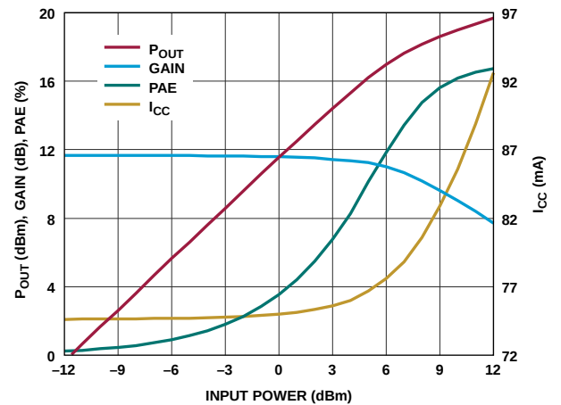
Figure 23. P_{OUT} , Gain, PAE, and I_{CC} vs. Input Power, Frequency = 7 GHz
