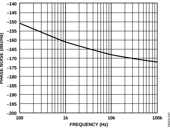
Figure 37. Phase Noise vs. Frequency at 10 GHz, P OUT = 10 dBm
