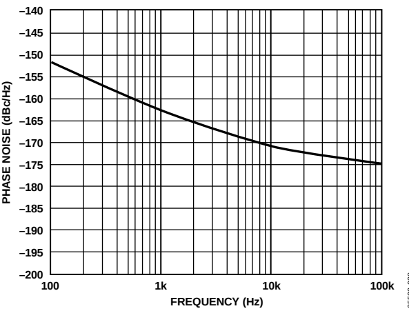
Figure 38. Phase Noise vs. Frequency at 10 GHz, P OUT = P SAT
