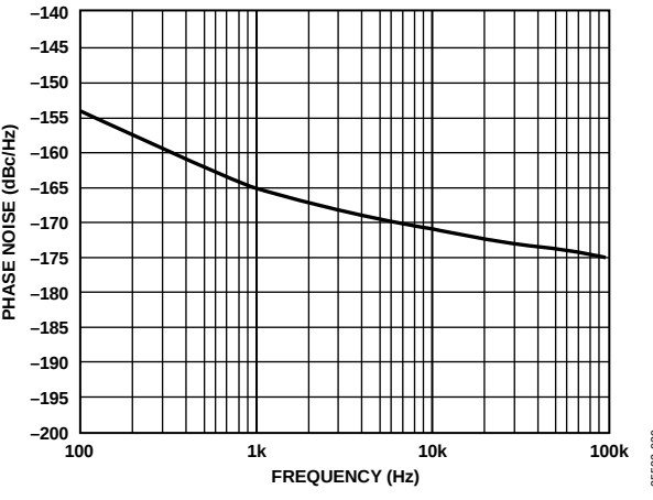
Figure 39. Phase Noise vs. Frequency at 10 GHz, P OUT = P 1dB
