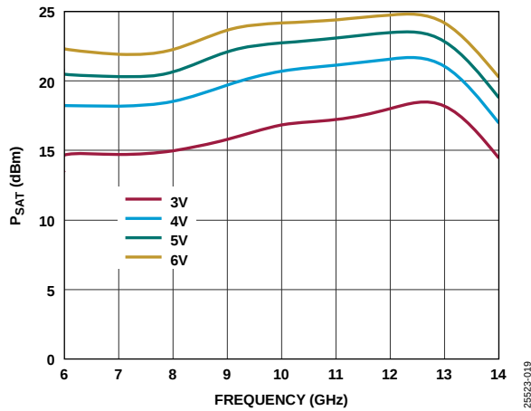
Figure 19. P_{SAT} vs. Frequency for Various Supply Voltages
