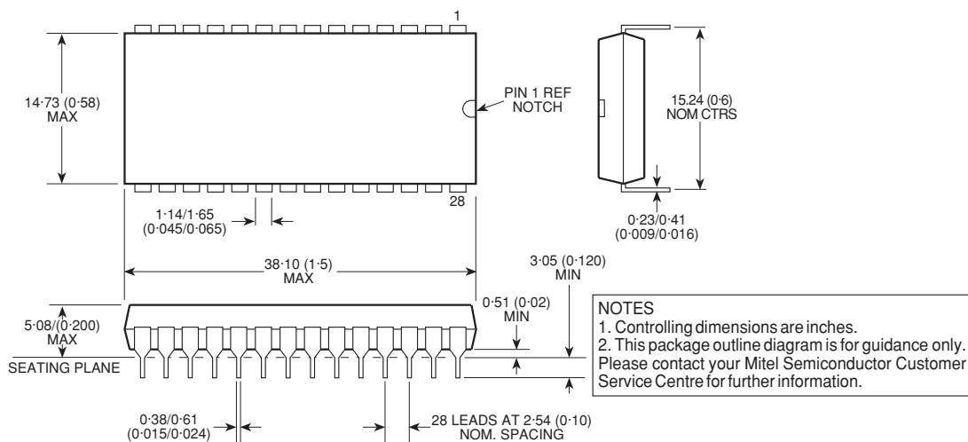
28-LEAD PLASTIC DIL - DP28
