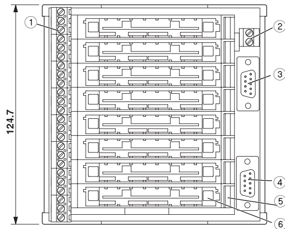
Figure 1 Structure
