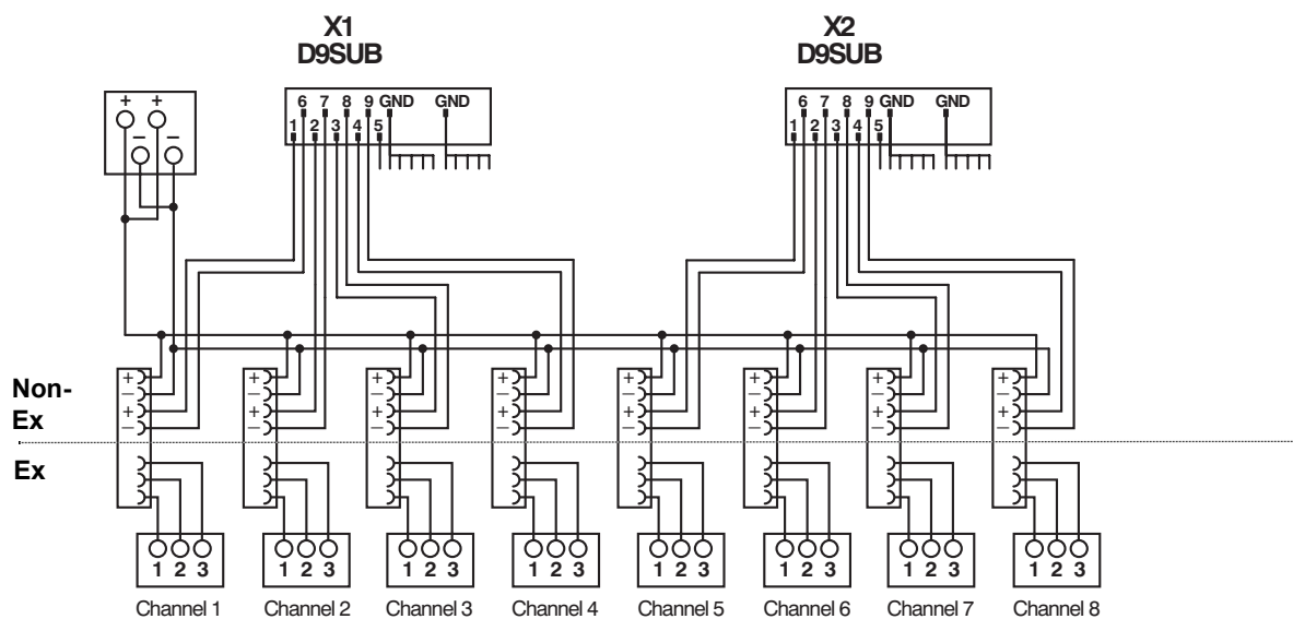
Figure 3 Circuit diagram
