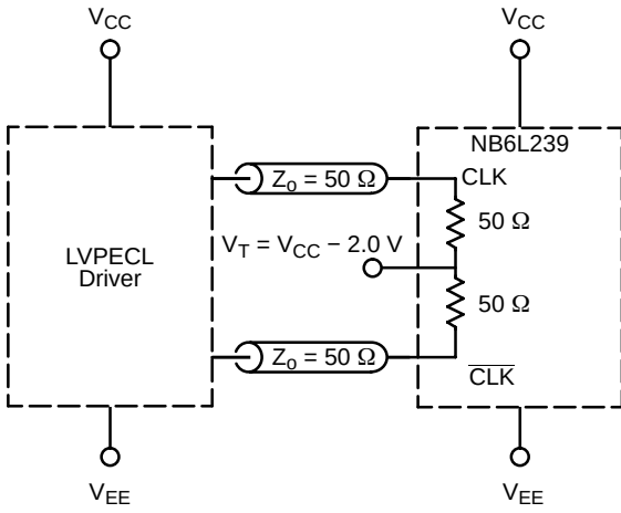
Figure 12. LVPECL Interface
