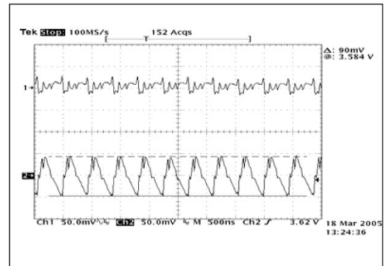
Fig. 9: Ripple 2x Flash 400mA, Ch1= V_{IN} , Ch2= V_{OUT} V_{IN}=3.6V , C_{IN}=4.7\mu F , C_{FC}=0.47\mu F , C_{OUT}=2.2\mu F
