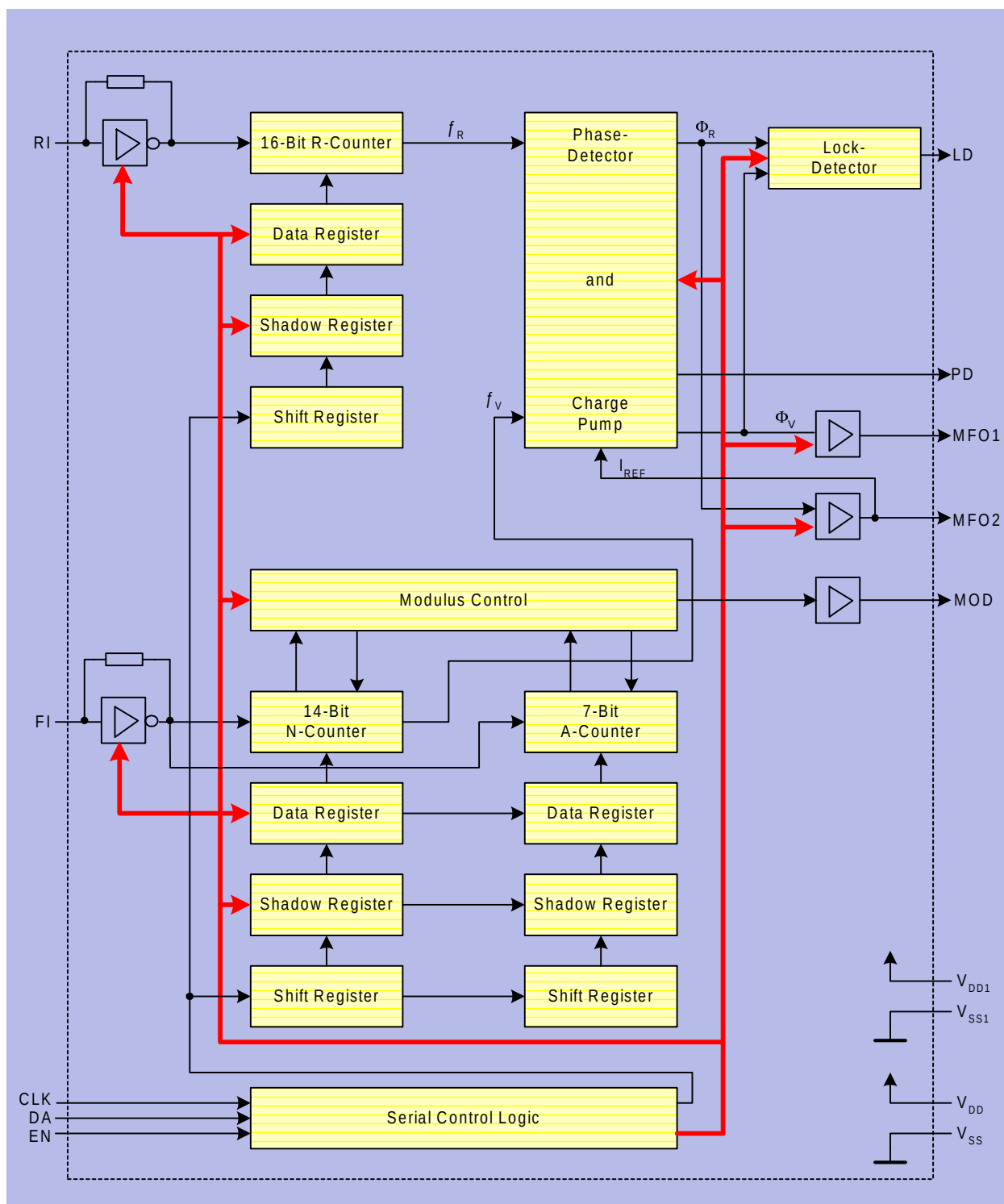
Figure 3-2 Functional Block Diagram
