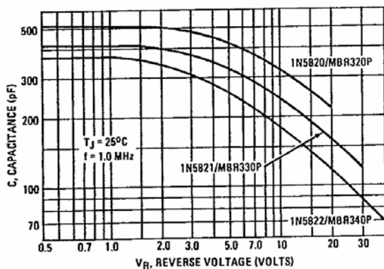
FIGURE 11 – TYPICAL CAPACITANCE
