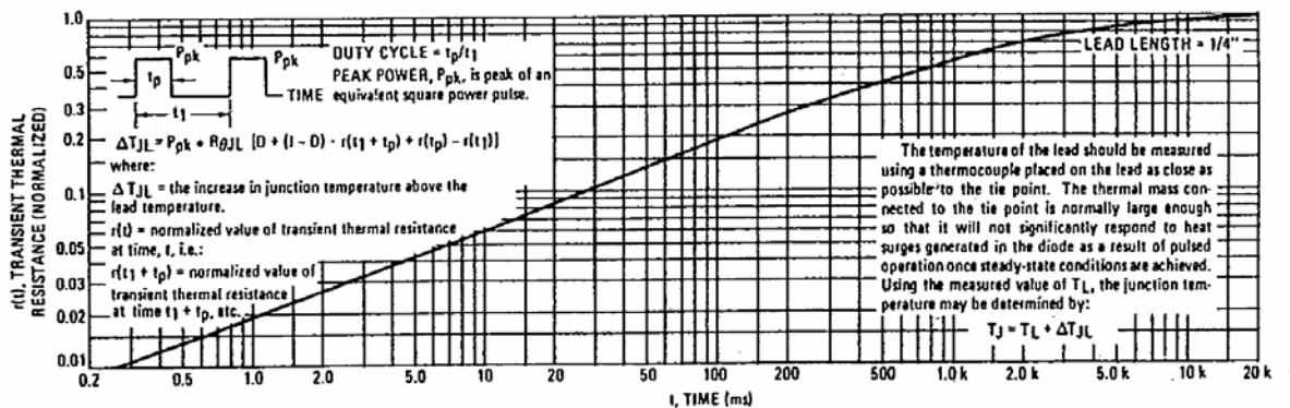
FIGURE 5 -- THERMAL RESPONSE
