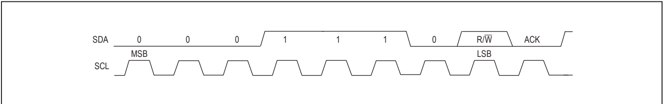
Figure 10. Slave Address
