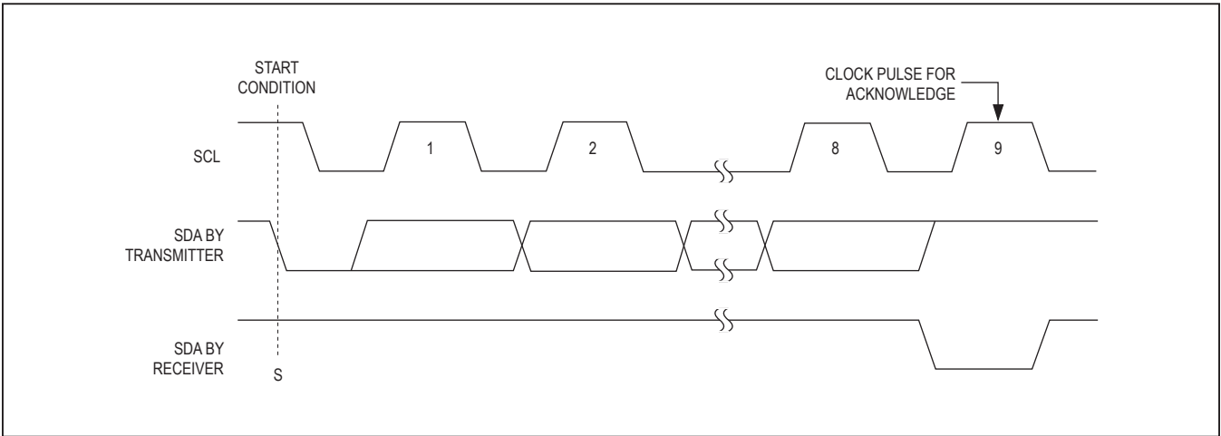
Figure 9. Acknowledge
