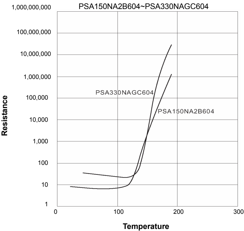
R-T Characteristic Curve (Representative)
