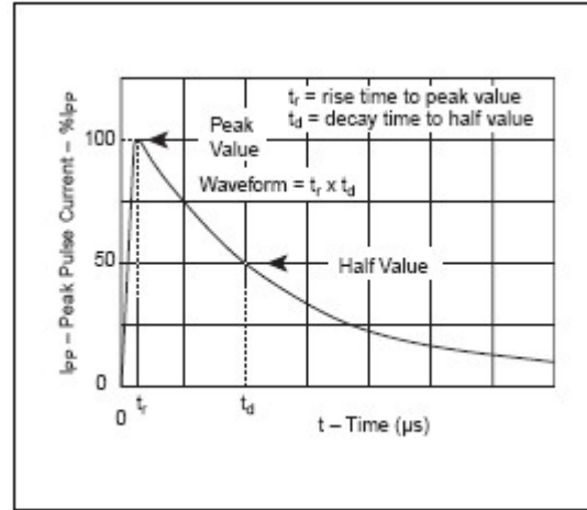
Fig 2. t_r \times t_d Pulse Waveform
