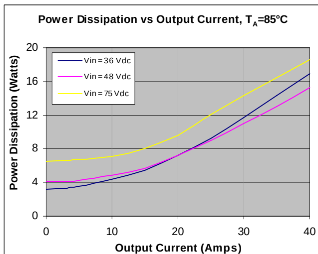
Figure 8. Power Dissipation vs. Load Current at T_A=85^\circ\text{C} for different input voltages with 300LFM airflow directed from Pins 3 to 1.
