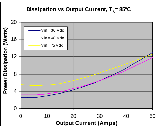
Figure 16. Power Dissipation vs. Load Current at T_A=85^{\circ}\text{C} for different input voltages with 300 LFM airflow directed from Pins 3 to 1.
