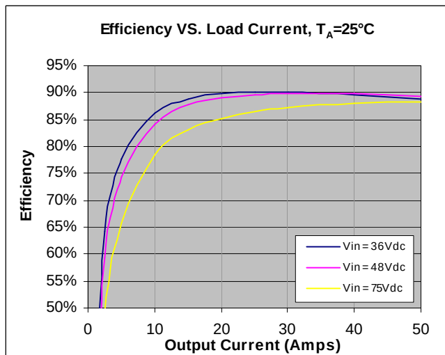
Figure 13. Efficiency vs. Load Current Curves at T_A=25^{\circ}\text{C} for different input voltages with 300 LFM airflow directed from Pins 3 to 1.
