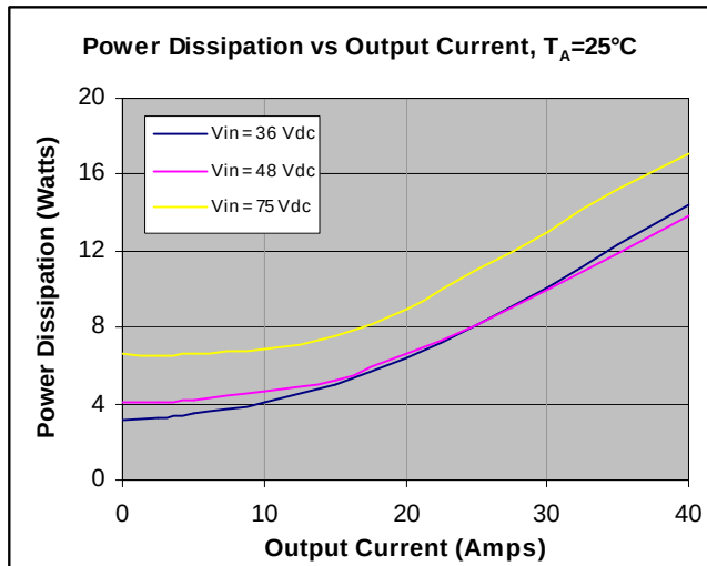
Figure 6. Power Dissipation vs. Load Current at T_A=25^\circ\text{C} for different input voltages with 300LFM airflow directed from Pins 3 to 1.
