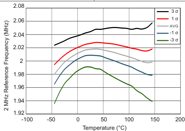
图 5-9. Oscillator Frequency (2MHz Reference, Divided Down from 250MHz) vs Temperature
