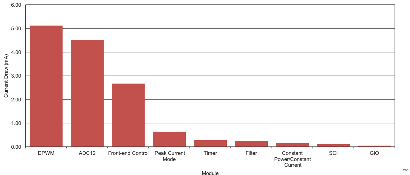
图 5-10. Clock Gating Power Savings
