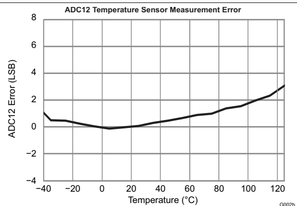
图 5-8. ADC12 Temperature Sensor Measurement Error vs Temperature
