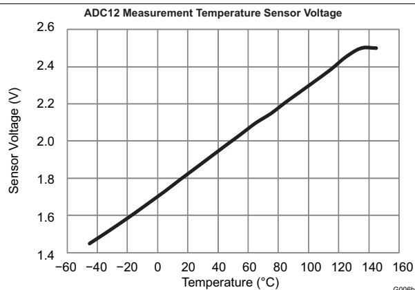
图 5-6. ADC12 Measurement Temperature Sensor Voltage vs Temperature
