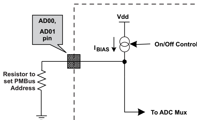
图 6-21. PMBUS Address Detection Method
