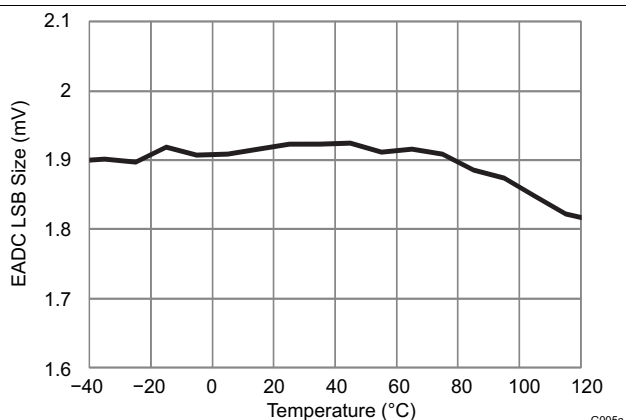
图 5-5. EADC LSB Size with 4X Gain (mV) vs Temperature
