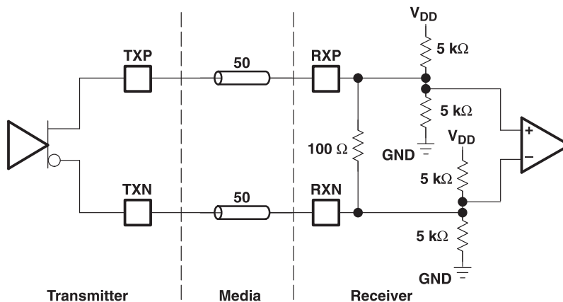
Figure 9. High-Speed I/O Directly-Coupled Mode
