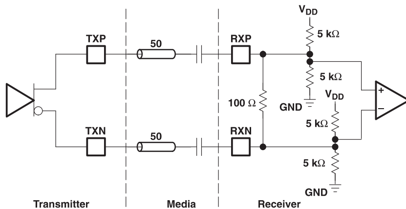
Figure 10. High-Speed I/O AC-Coupled Mode
