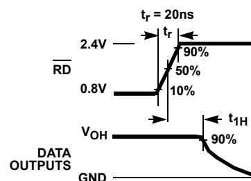
FIGURE 1B. t_{1H} , C_I = 10\text{pF}
