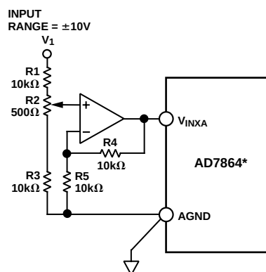
Figure 13. Full-Scale Adjust Circuit
