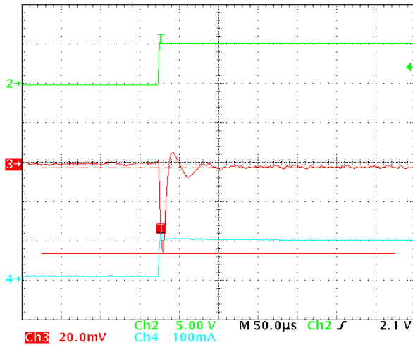
Figure 17. 10 mA to 100 mA Load Transient in 1 \mu\text{s} ( V_{IN} = 3.6 \text{ V} , V_{OUT} = 1.2 \text{ V} , Temperature = 25^\circ\text{C} )
