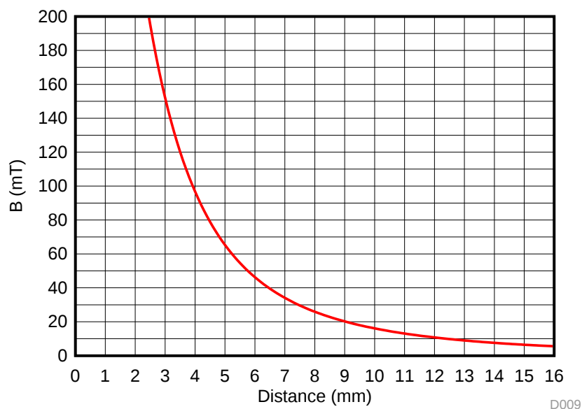
Figure 22. Magnetic Field vs Distance
