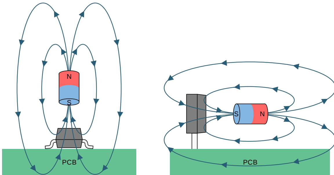
Figure 13. Flux Direction for Positive B
