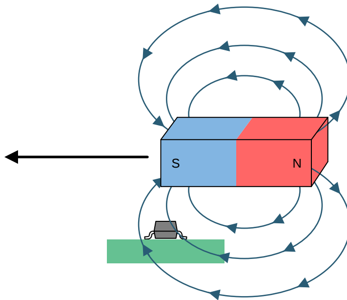
Figure 18. Common Magnet Orientation
