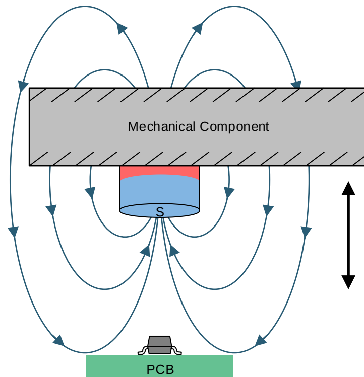
Figure 20. Physical Setup
