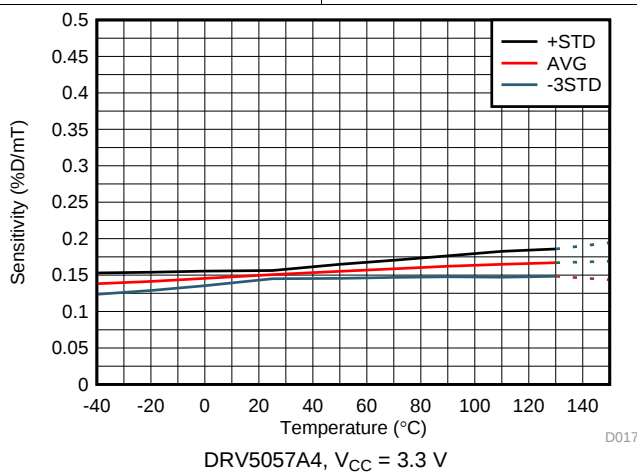
Figure 11. Sensitivity vs Temperature
