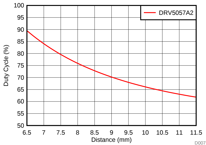
Figure 24. %D vs South Pole Distance (Gain A2)
