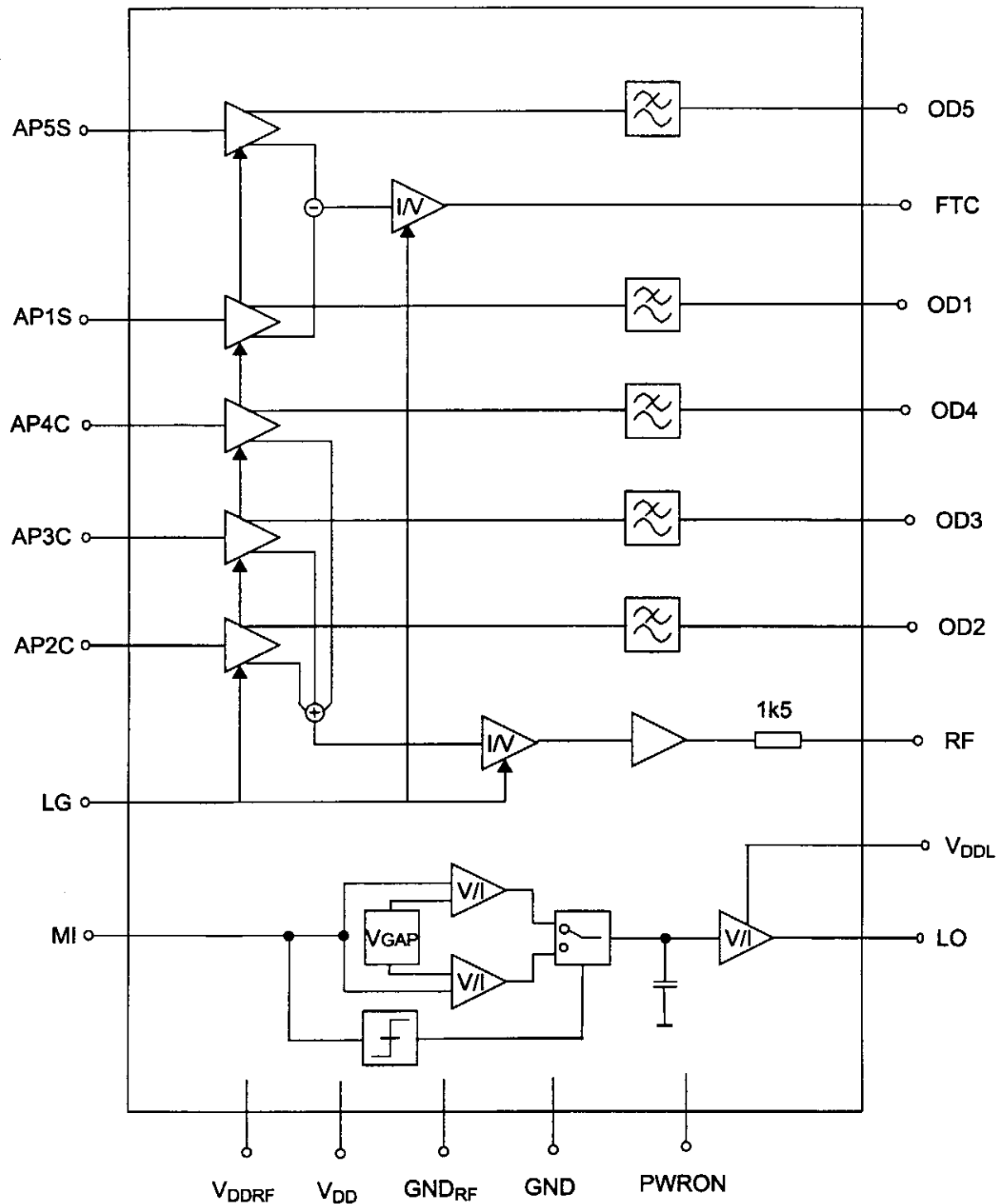
Fig.1 Block diagram
