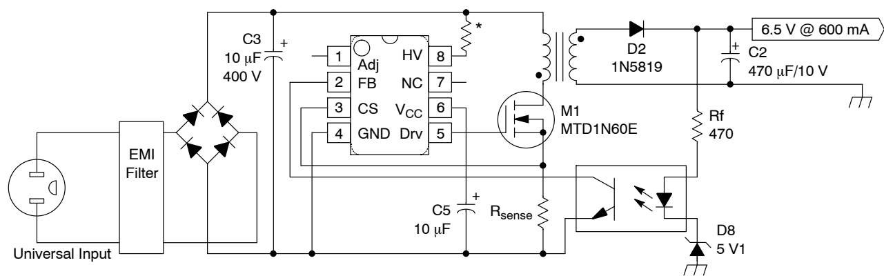
Figure 1. Typical Application
