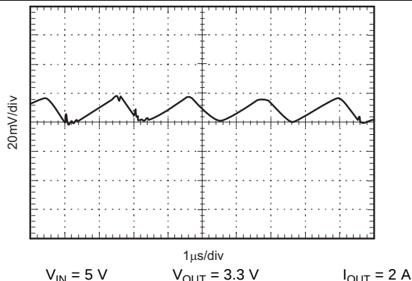
Figure 20. Buck Output Voltage Ripple
