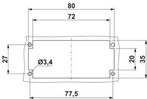
Mounting cut-out
