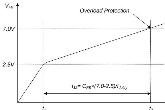
Figure 21. Overload Protection
