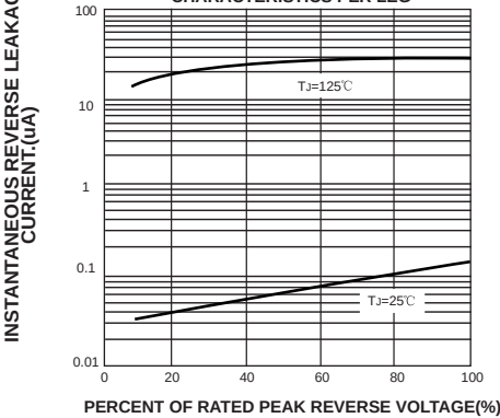
FIG. 4-TYPICAL REVERSE LEAKAGE CHARACTERISTICS PER LEG
