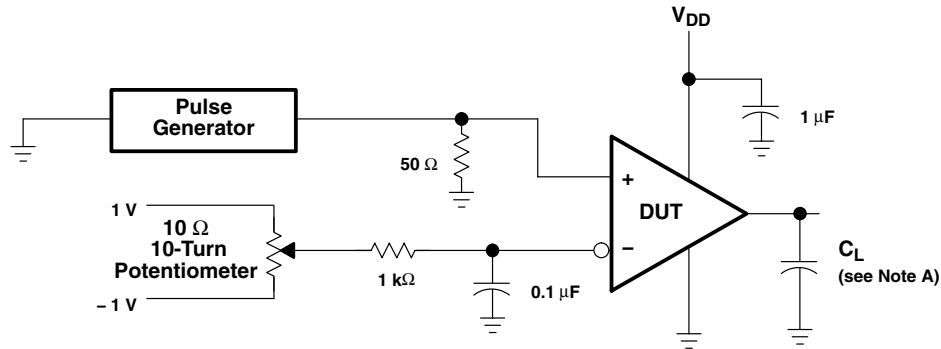
TEST CIRCUIT
