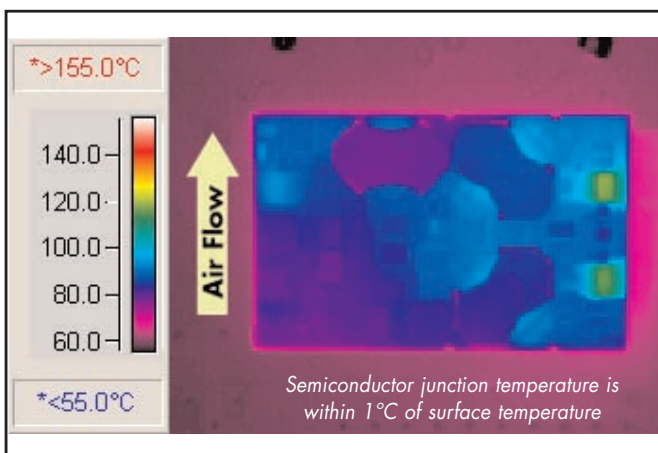
Figure 8: Thermal plot of converter at 15 amp load current with 55°C air flowing at the rate of 200 LFM. Air is flowing across the converter from pin 3 to pin 1 (nominal input voltage).
