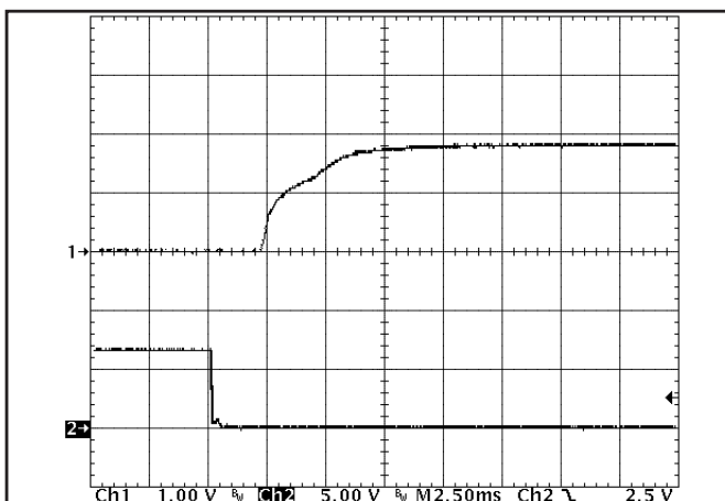
Figure 10: Turn-on transient at zero load (2.5 ms/div). Ch1: V_{out} (1V/div). Ch2: ON/OFF input (5V/div).
