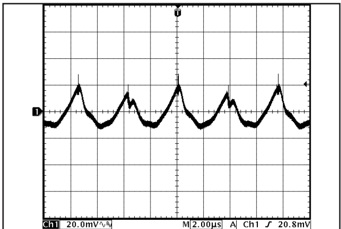
Figure 16: Output voltage ripple at nominal input voltage and rated load current (20 mV/div). Load capacitance: 1\ \mu F ceramic capacitor and 15\ \mu F tantalum capacitor. Bandwidth: 20 MHz. See Figure 13.
