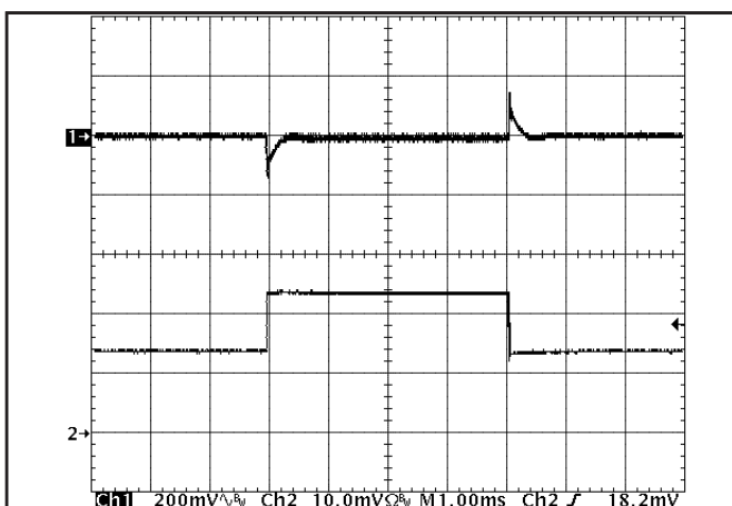
Figure 12: Output voltage response to step-change in load current (50%-75%-50% of I_{out(max)} ; dI/dt = 5A/\mu s ). Load cap: 470 \mu F , 30 m \Omega ESR tantalum capacitor and 1 \mu F ceramic cap. Ch1: V_{out} (200mV/div), Ch2: I_{out} (5A/div).
