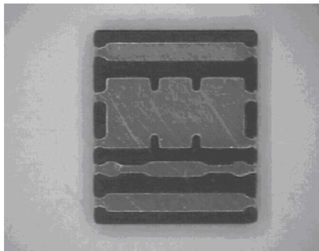
Figure 2: Bottom View of a PolarPAK
