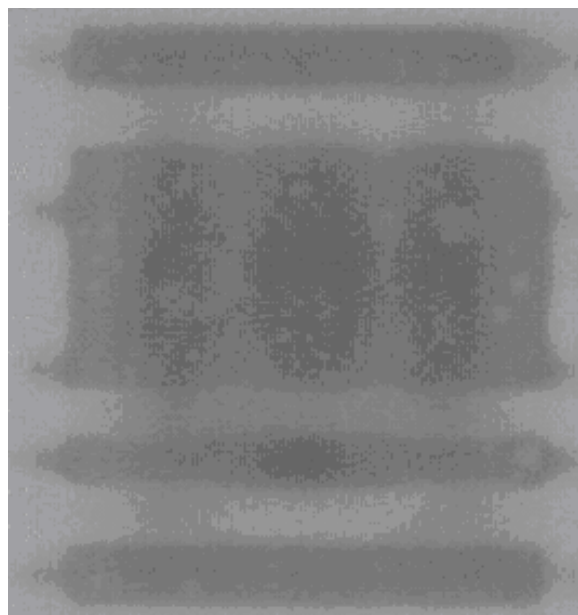
Largest void Board#: 32 Location: U14
