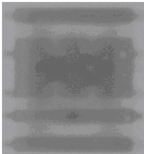
Smallest void Board#: 32 Location: U11
