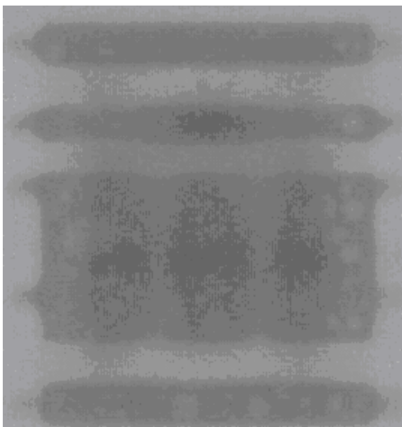
Largest void Board#: 31 Location: U10
