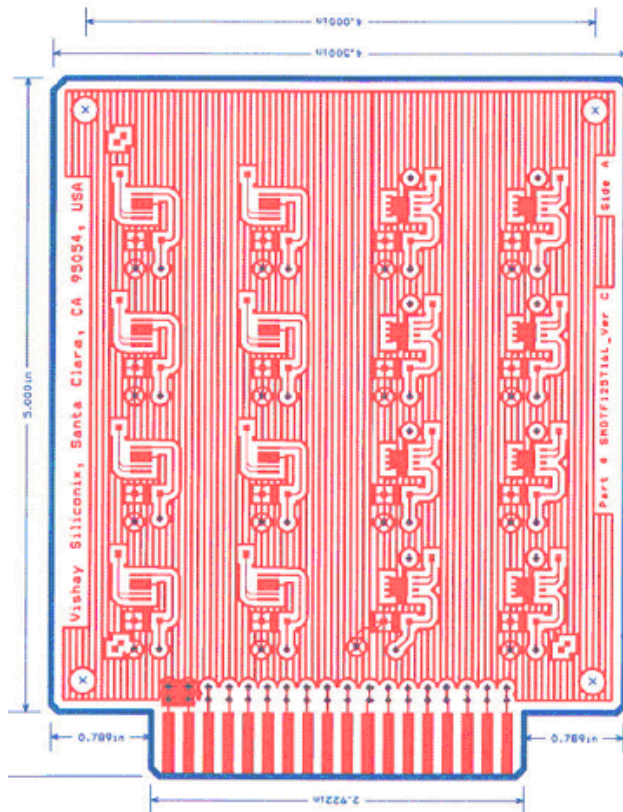
Figure 6 PCB Dimensions
