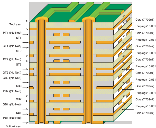
Figure 3: PCB Layer-Stack
