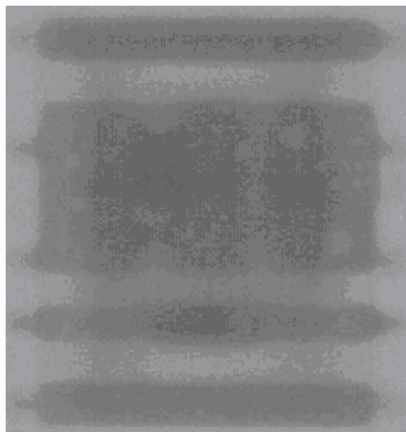
Smallest void Board#: 34 Location: U13
