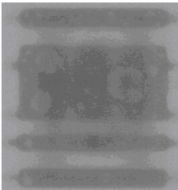
Largest void Board#: 34 Location: U14
