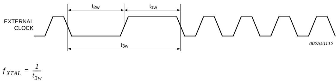
Fig 9. External clock timing
