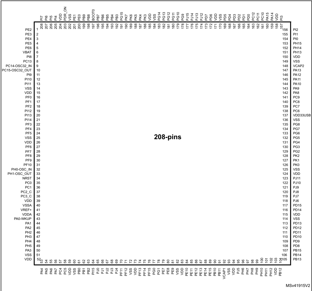
Figure 9. LQFP208 pinout
