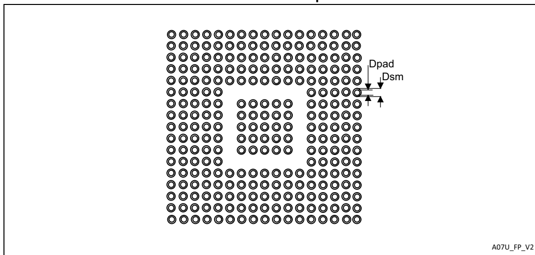
Figure 83. TFBGA240+25 - 265 pin pin, 14x14 mm 0.8 mm pitch recommended footprint
