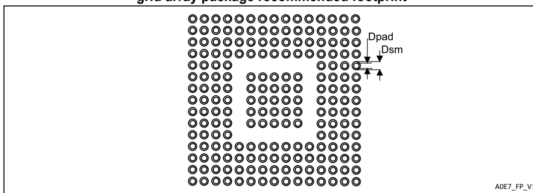
Figure 80. UFBGA176+25 - 201-ball, 10 x 10 mm, 0.65 mm pitch, ultra fine pitch ball grid array package recommended footprint
