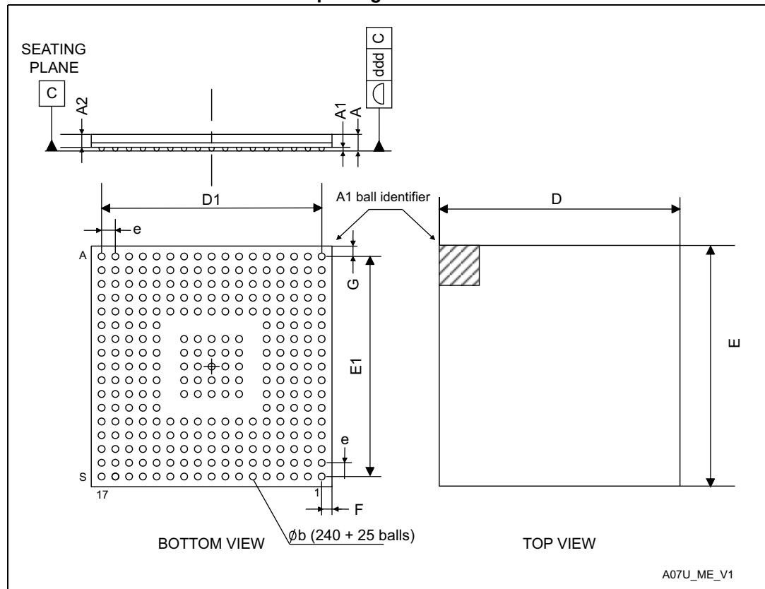
Figure 82. TFBGA240+25 - 265 pin, 14x14 mm, 0.8 mm pitch, fine pitch ball grid array package outline
