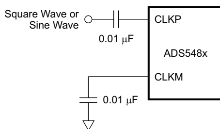
Figure 40. Single-Ended Clock
