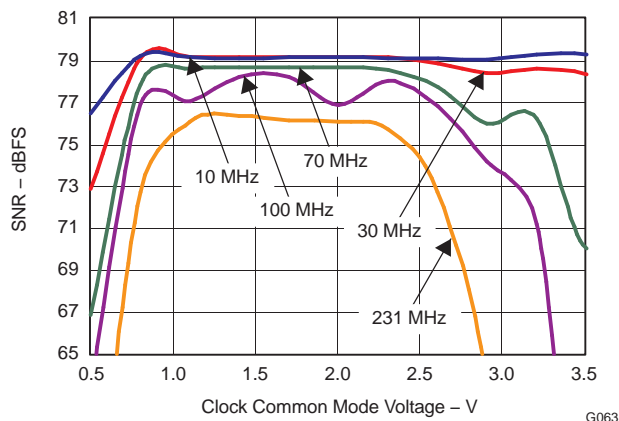
Figure 45. SNR versus Clock Common Mode
