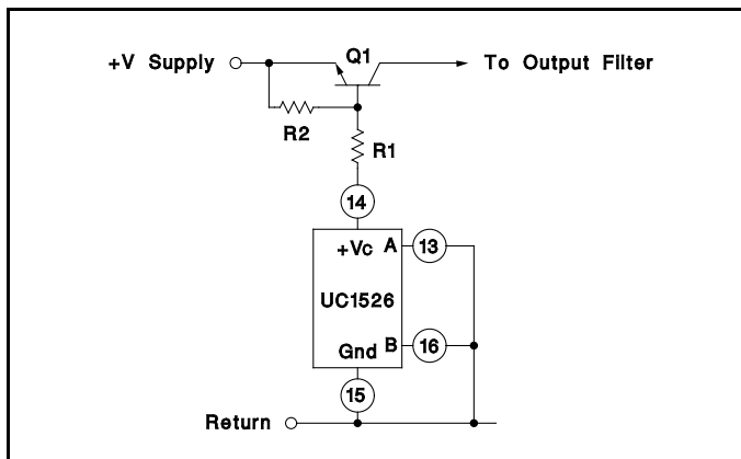
Figure 8. Single-Ended Configuration
