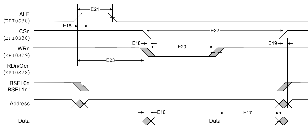
Figure 32-22. Host-Bus 8/16 Asynchronous Mode Write Timing
