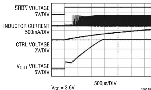
Figure 5. Soft-Start Waveform
