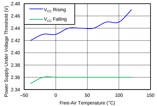
Figure 12. V<sub>CC</sub> UNDERVOLTAGE THRESHOLD vs FREE-AIR TEMPERATURE
