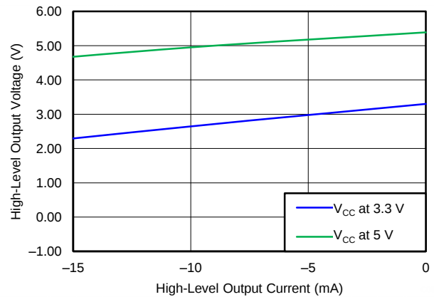
Figure 10. HIGH-LEVEL OUTPUT VOLTAGE vs HIGH-LEVEL OUTPUT CURRENT
