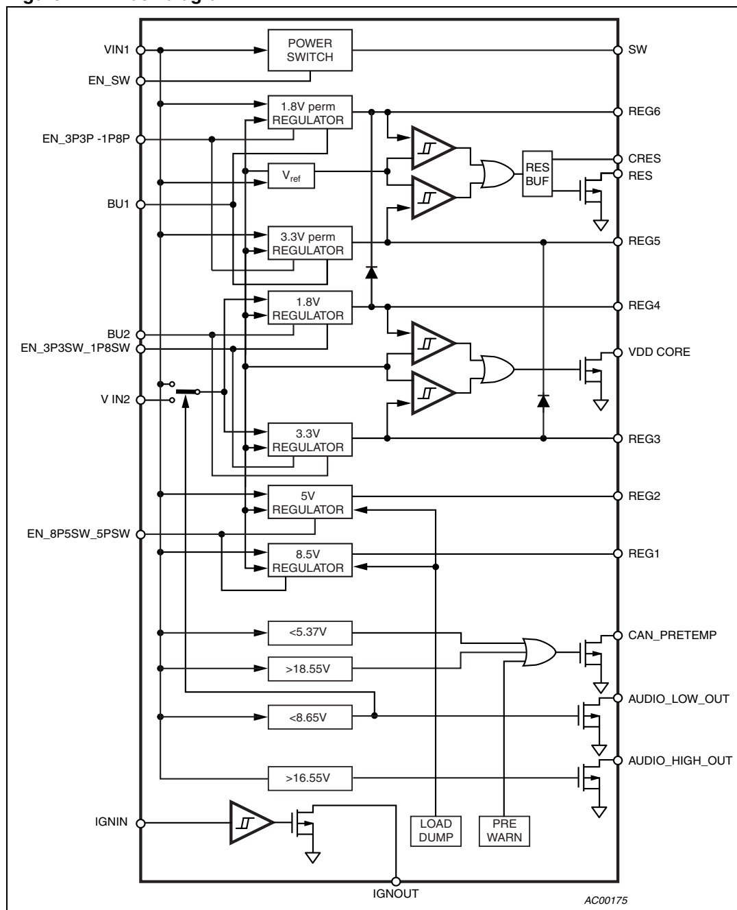
Figure 1. Block diagram
