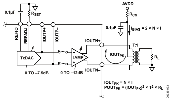
Figure 23. Current-Mode Operation
