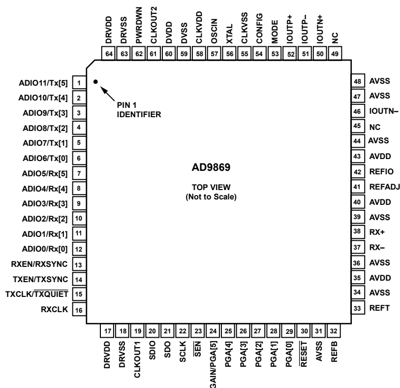
Figure 2. Pin Configuration
