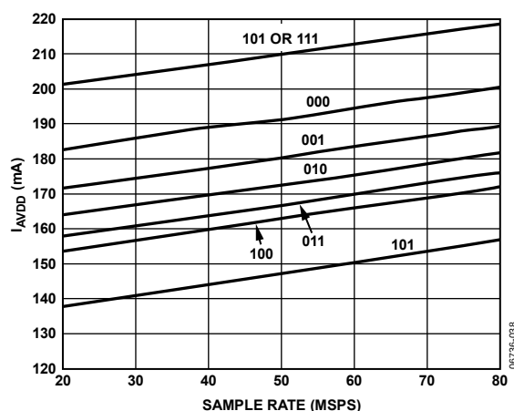
Figure 38. AVDD Current vs. ADC Bias Setting and Sample Rate
