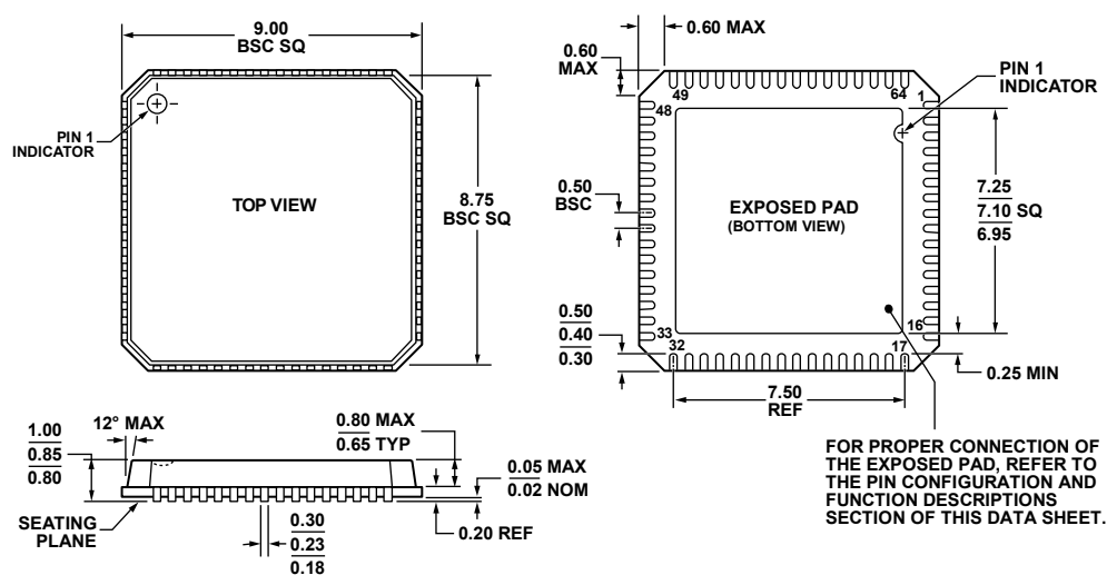
Figure 40. 64-Lead Lead Frame Chip Scale Package [LFCSP_VQ]
